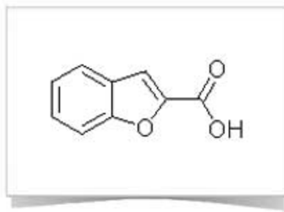
Benzofuran-2-Carboxylic Acid
