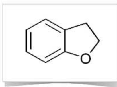
dihydrobenzofuran
