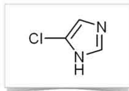
5-chloroimidazole
