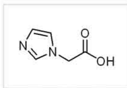
Imidazol-1-yl-acetic acid
