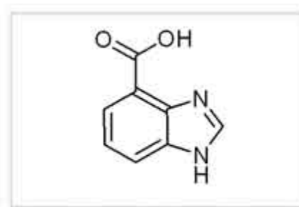
1H-benzimidazole-4-carboxylic acid
