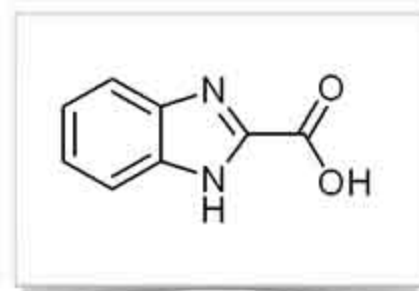
1H-Benzimidazole-2-carboxylic acid
