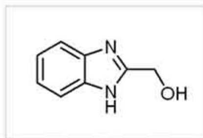
2 - hydroxymethylbenzimidazole
