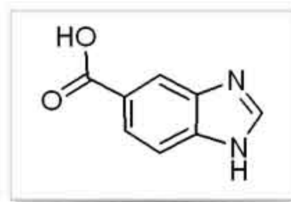
1H-Benzimidazole-5-carboxylic acid
