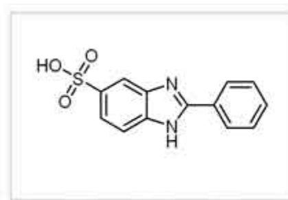
2-phenylbenzimidazole-5-sulphonic acid
