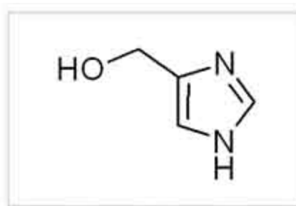
4-hydroxymethyl)imidazole
