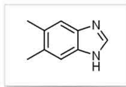
5,6-Dimethylbenzimidazole
