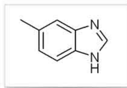
5-methylbenzimidazole
