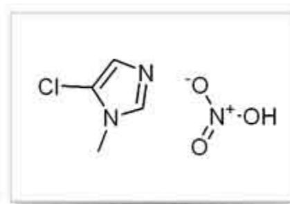
1-methyl-5-chloroimidazole nitrate
