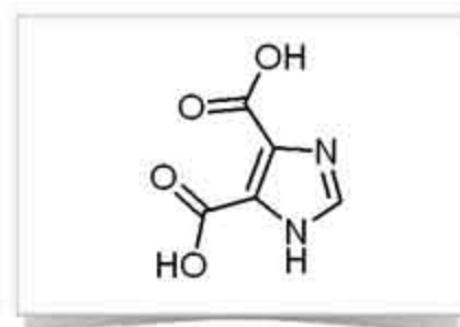
Imidazole-4,5-dicarboxylic acid
