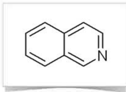
Isoquinoline
