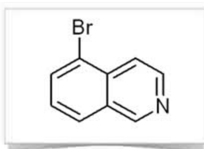
5-Bromoisoquinoline
