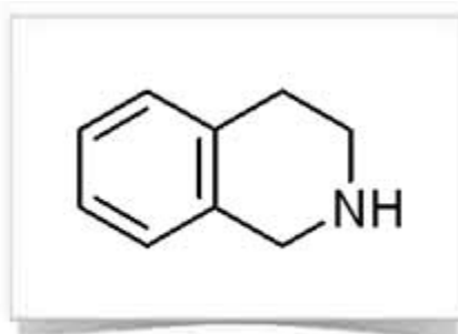
1,2,3,4-Tetrahydroisoquinoline CAS : 91-21-4
