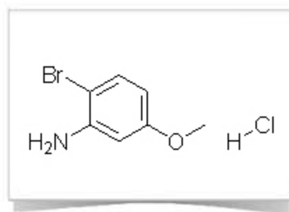
3-Amino-4-bromoanisole hydrochloride
