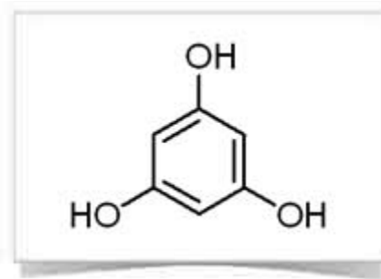
Phloroglucinol
