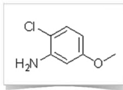
6-Chloro-m-Anisidine
