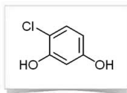
4-Chlororesorcinol
